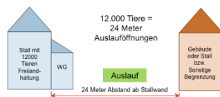
Figure 4: Example of corridor/minimum dimensions of free-range area
